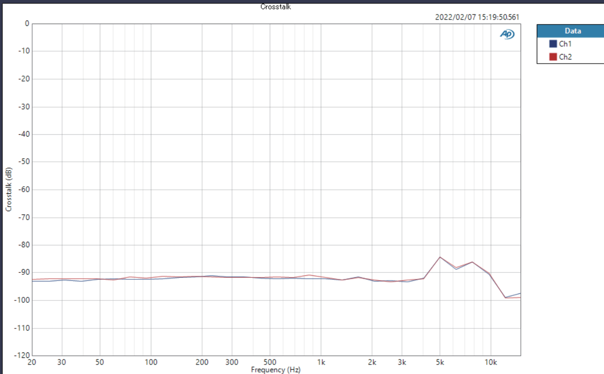
-35dBFS Sweep Crosstalk
