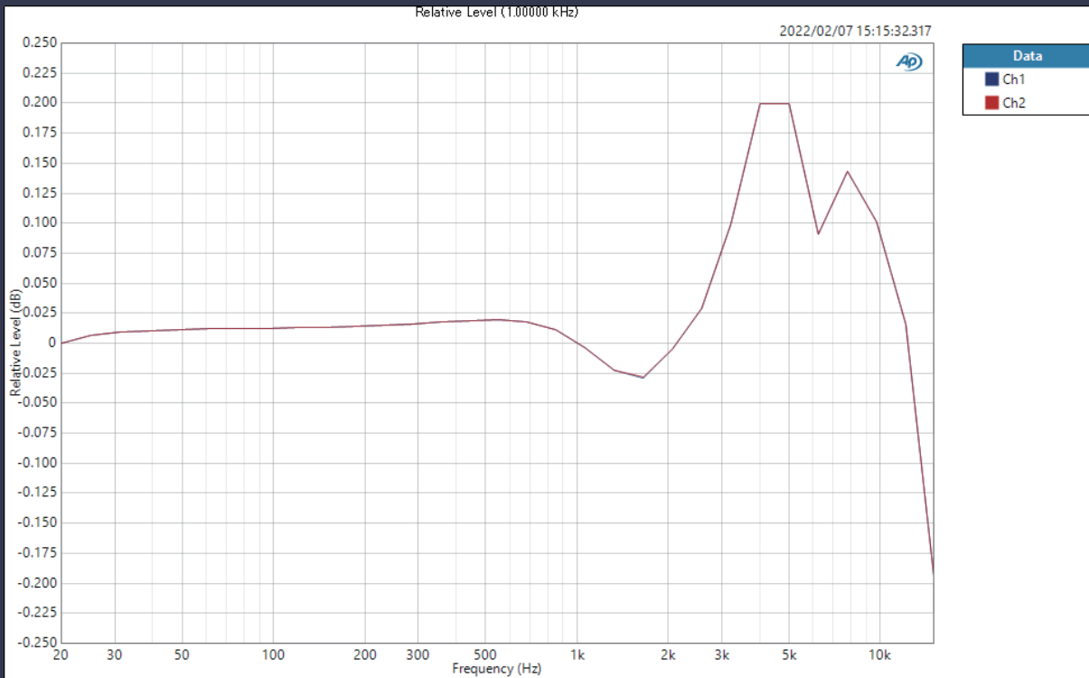
-35dBFS Sweep Relative Level (1.00000 kHz)
