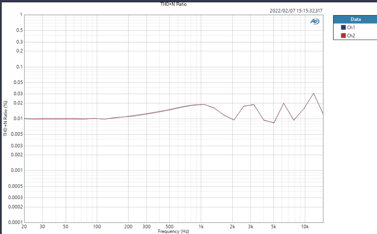
-35dBFS Sweep THD+N Ratio
